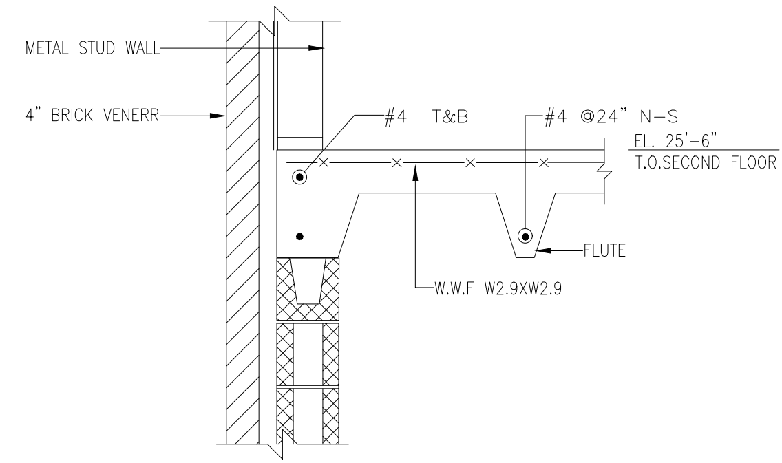
SECTION 2 SCALE - 3/4"=1'-0" REF:8/SD2.0
