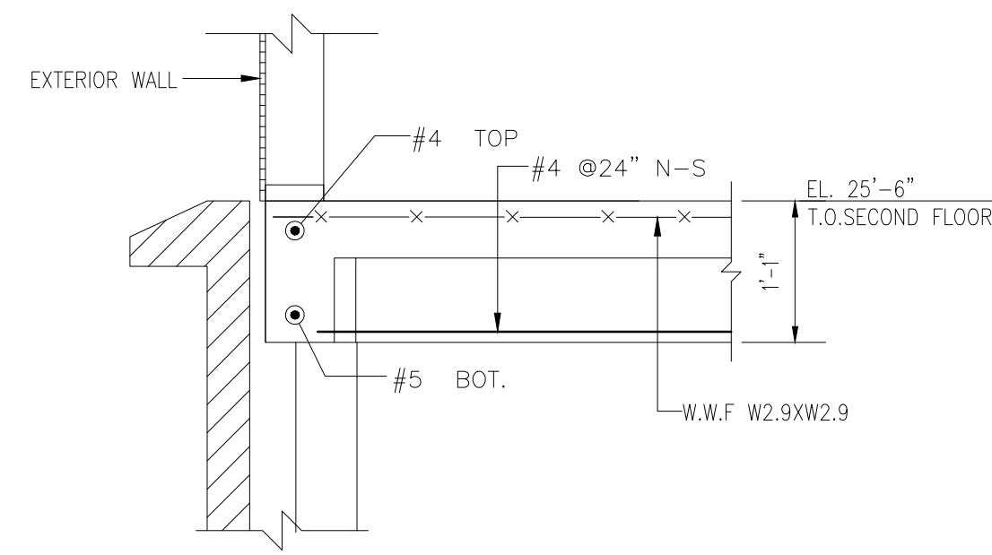
SECTION 3 SCALE - 3/4"=1'-0" REF:2B/SD2.0
