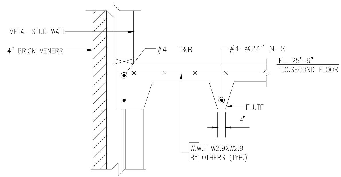
SECTION 1 SCALE - 3/4"=1'-0" REF:1A/SD2.0
