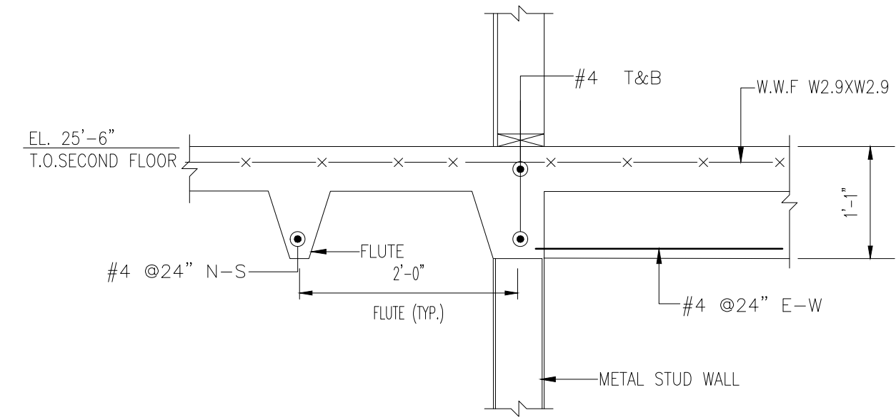
SECTION 5 SCALE - 3/4"=1'-0" REF:7/SD2.0
