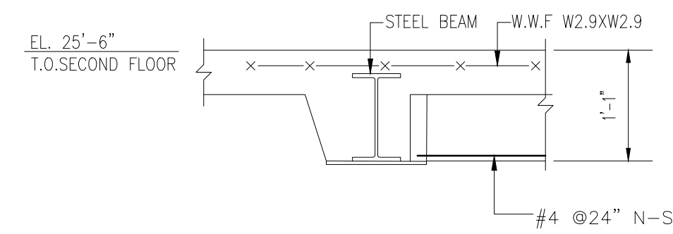
SECTION 7 SCALE - 3/4"=1'-0" REF:17/SD2.0
