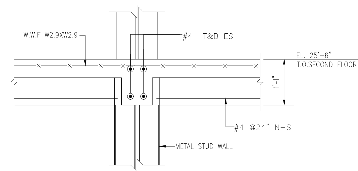
SECTION 6 SCALE - 3/4"=1'-0" REF:3/SD2.0
