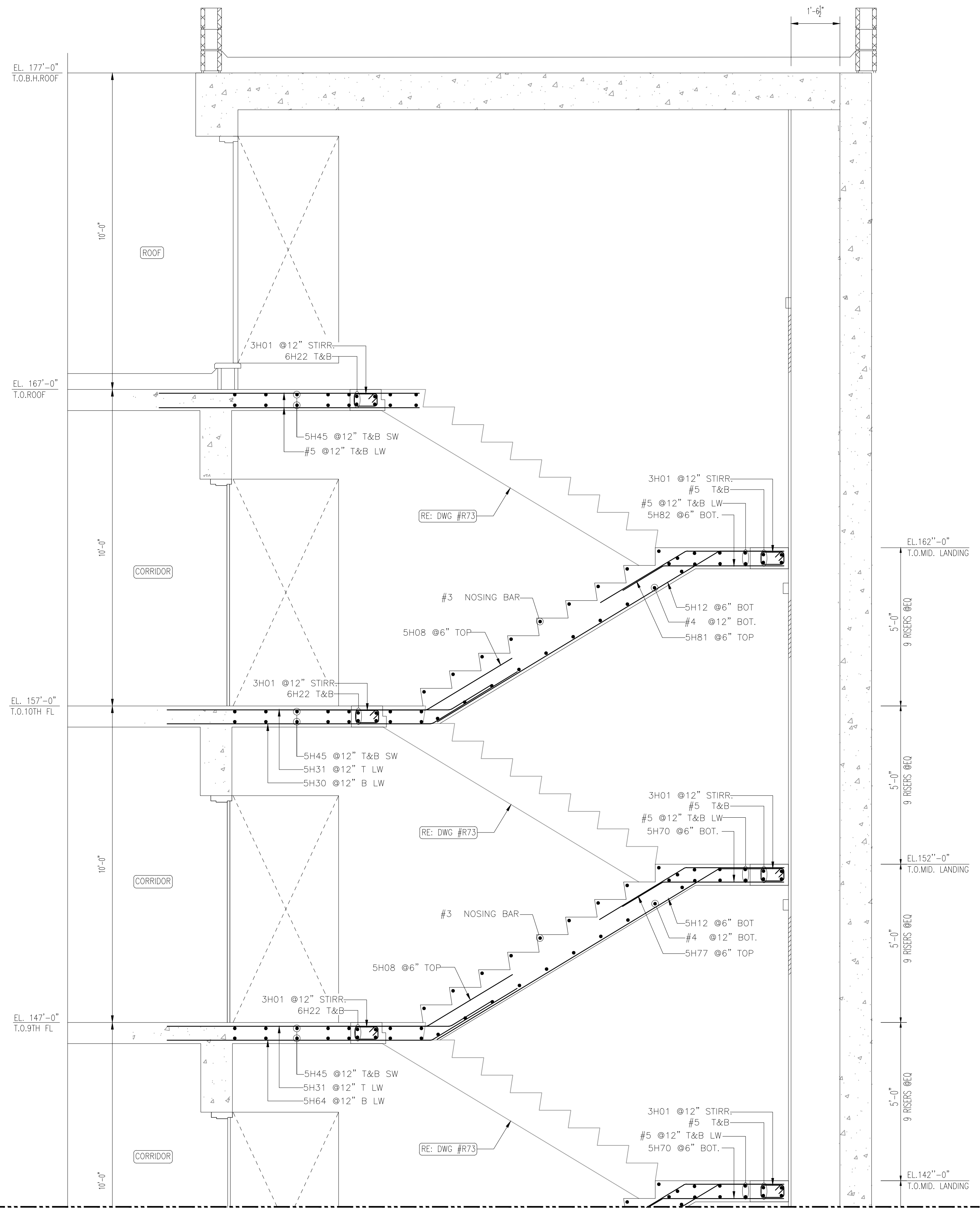
SECTION 1 SCALE- 1/2=1'-0" REF:S100 & S502
