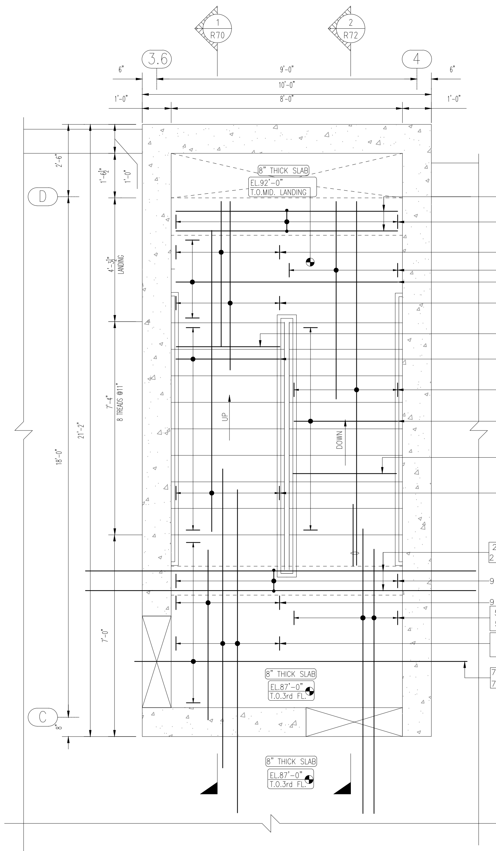
RESIDENTIAL LEVEL-3 DETAIL A SCALE- 1/2=1'-0" REF:S100 & S502
