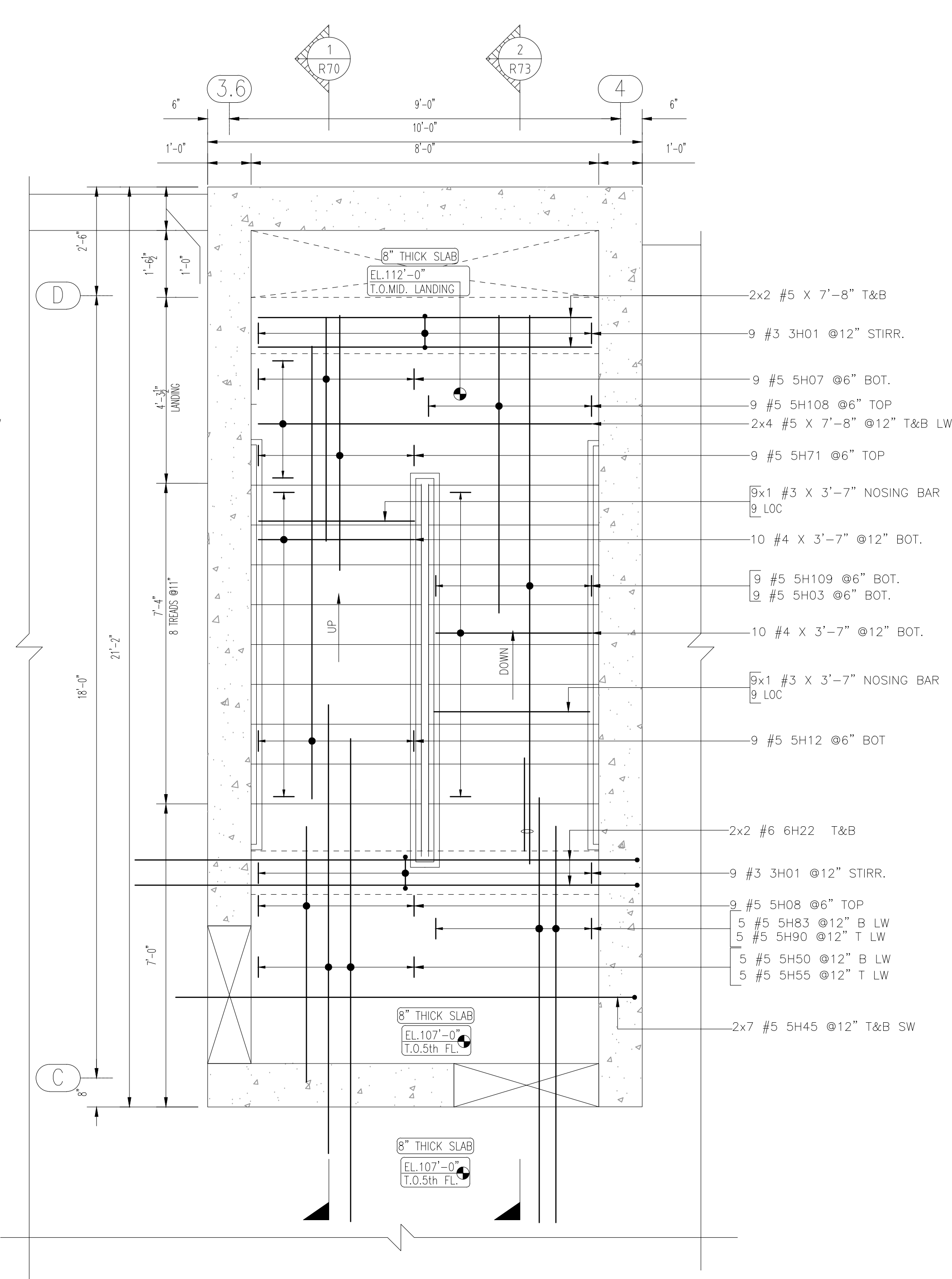
RESIDENTIAL LEVEL-5 DETAIL A SCALE- 1/2=1'-0" REF:S100 & S502
