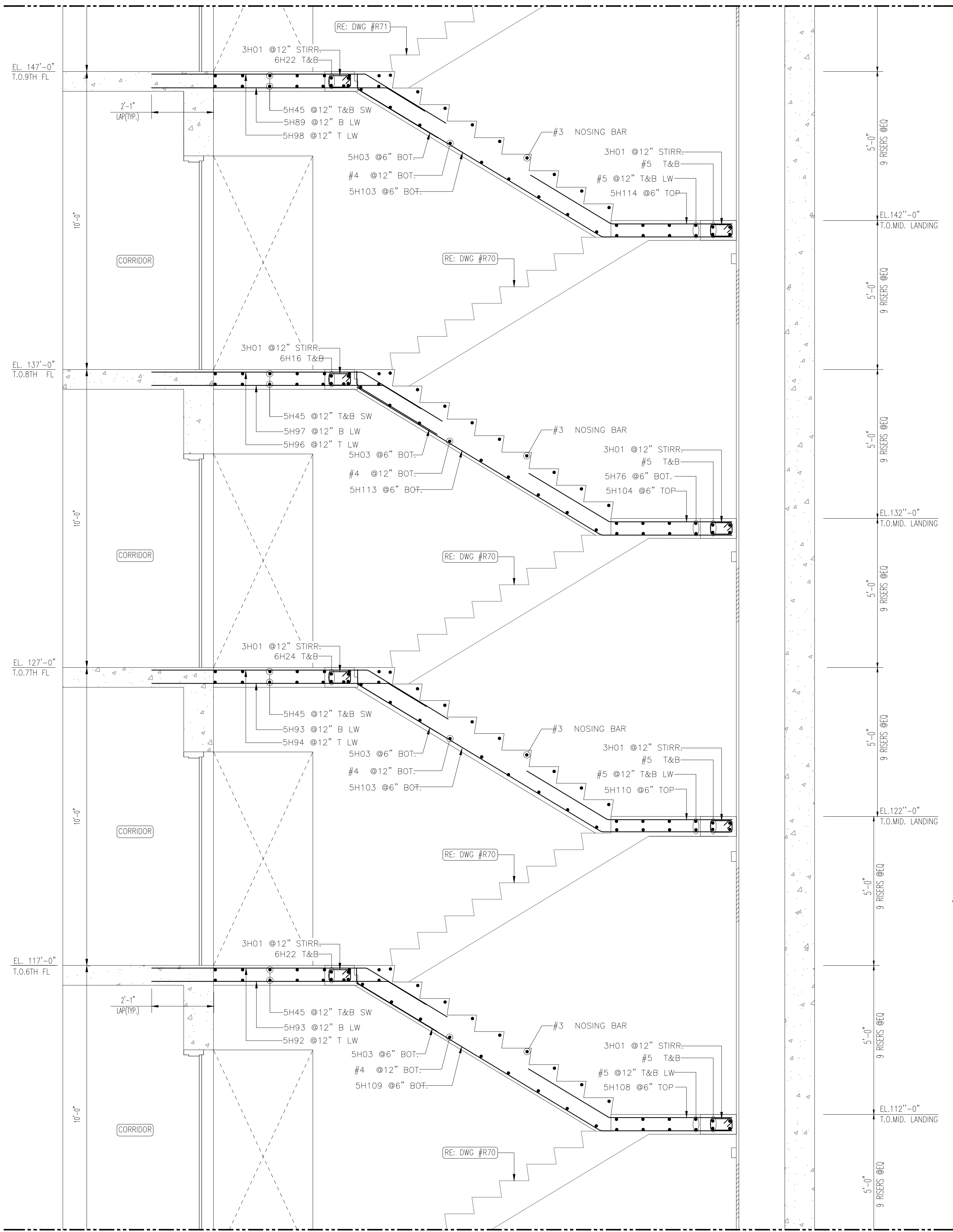
SECTION ② SCALE- 1/2=1'-0" REF:S100 & S502
