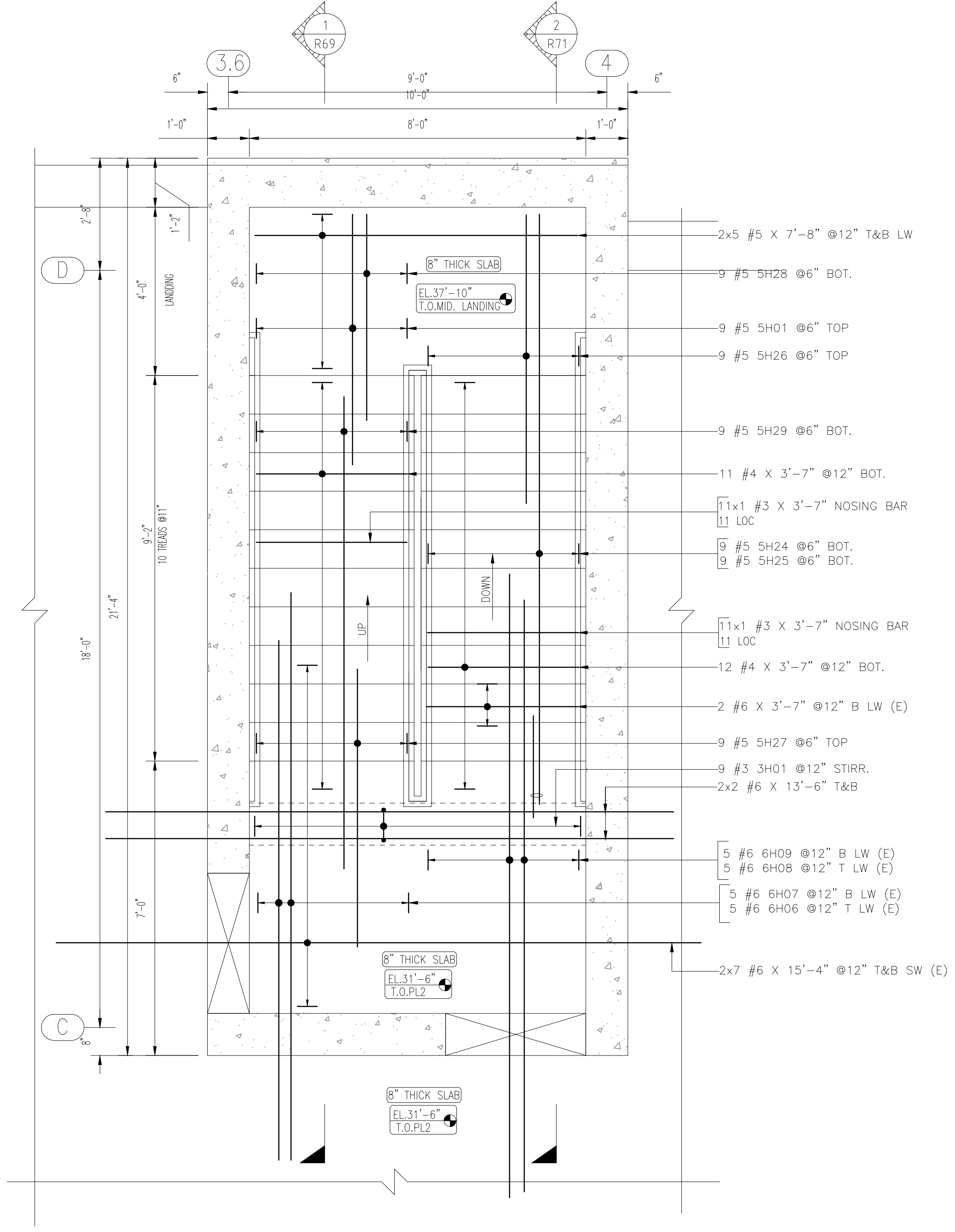
PARKING LEVEL-2 DETAIL A SCALE- 1/2=1'-0" REF:S100 & S502
