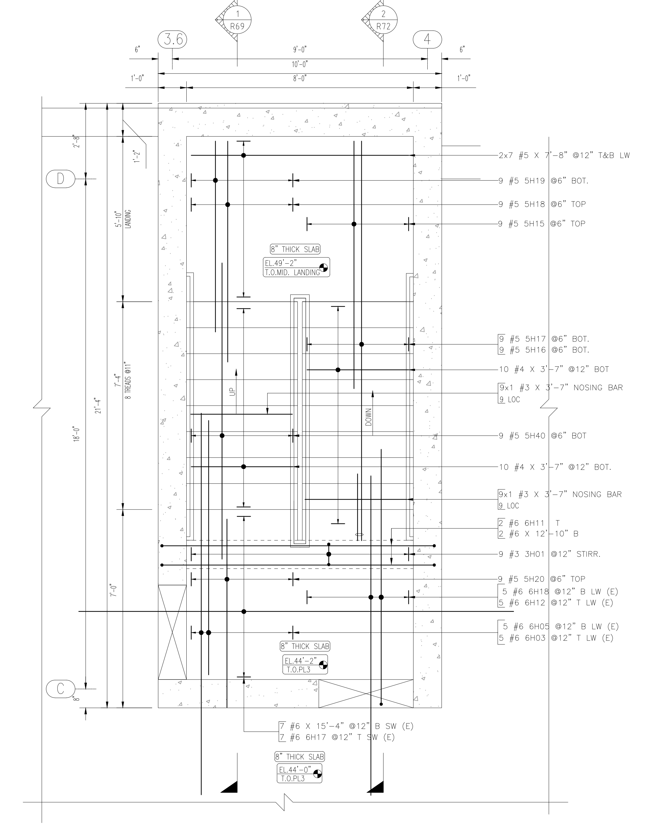
PARKING LEVEL-3 DETAIL A SCALE- 1/2=1'-0" REF:S100 & S502
