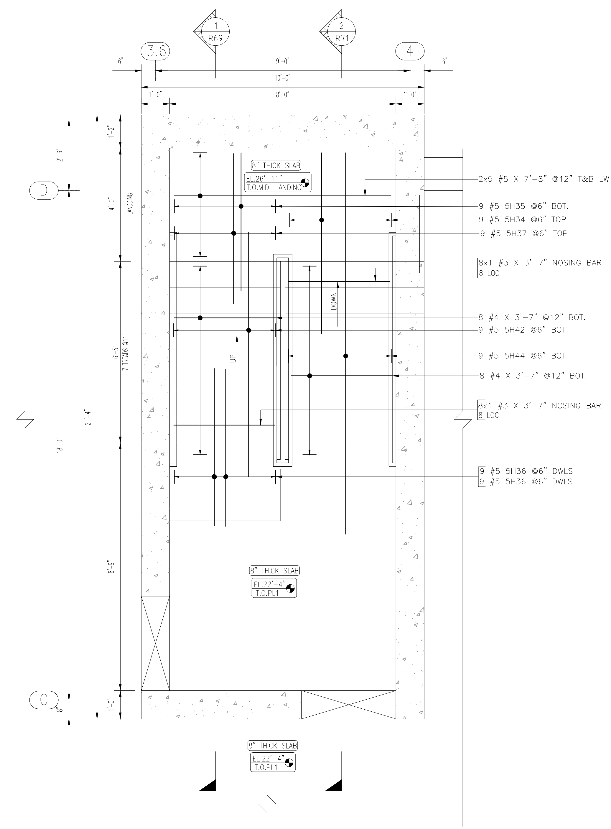
PARKING LEVEL-1 DETAIL A SCALE- 1/2=1'-0" REF:S100 & S502
