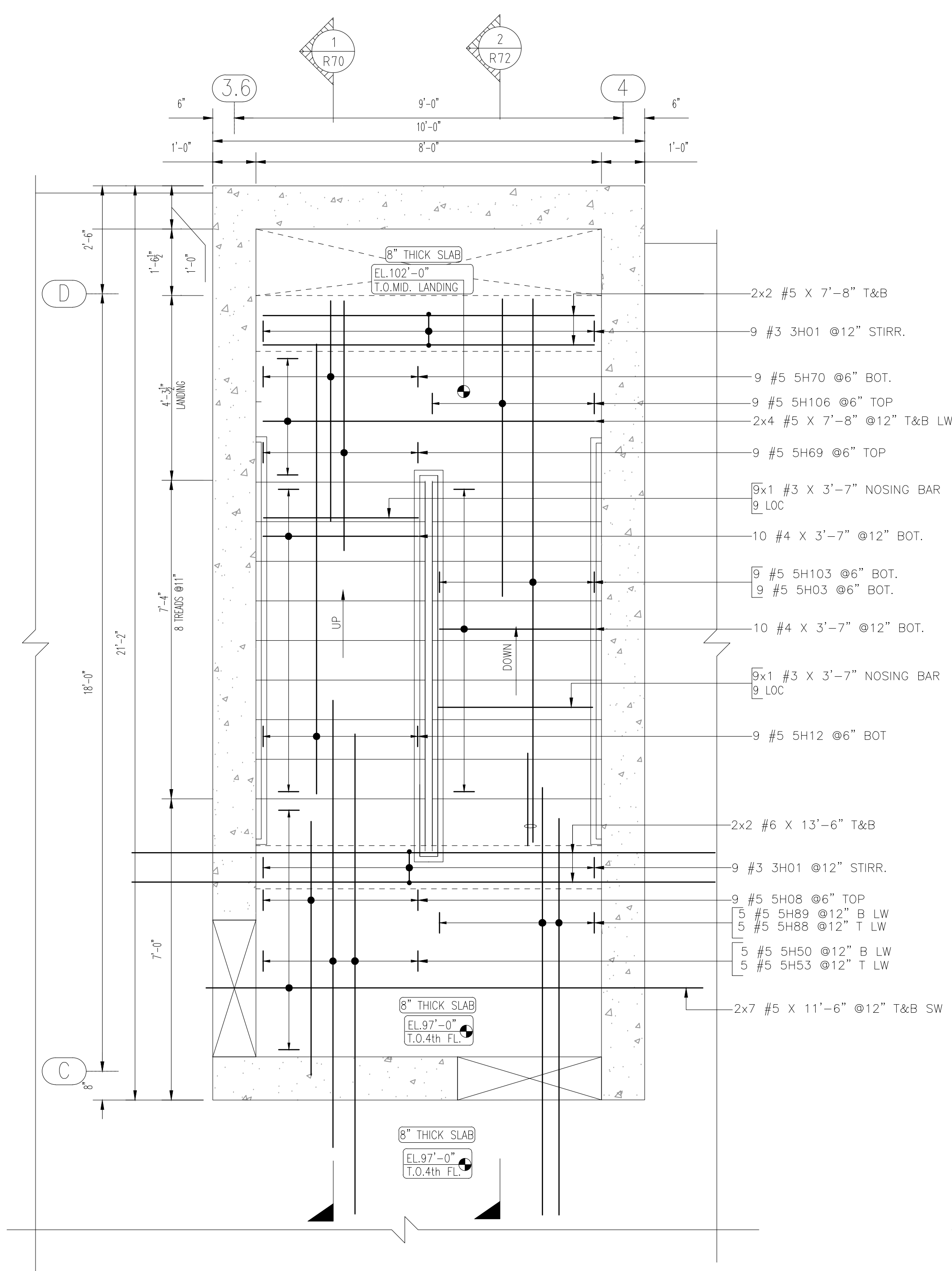
RESIDENTIAL LEVEL-4 DETAIL A SCALE- 1/2=1'-0" REF:S100 & S502
