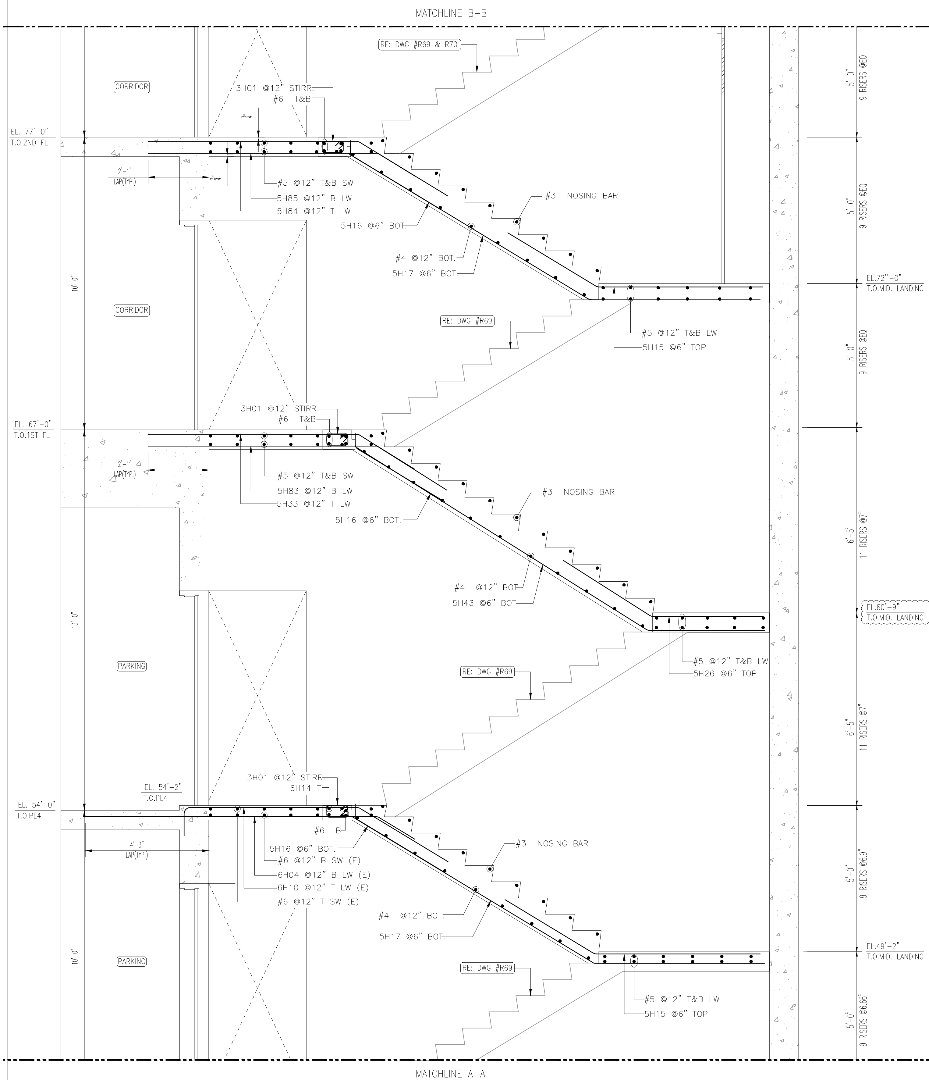
SECTION 2 SCALE- 1/2=1'-0" REF: S100 & S502
